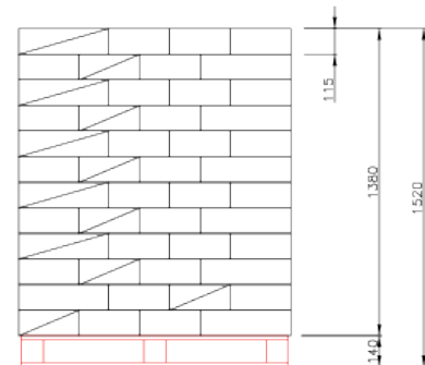
Pallet EPAL
