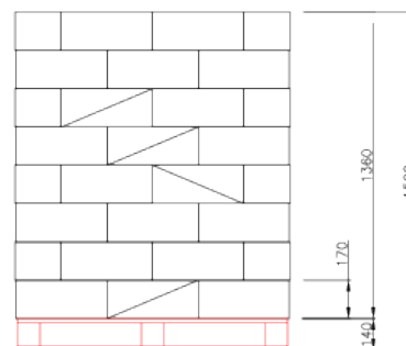
Pallet EPAL
