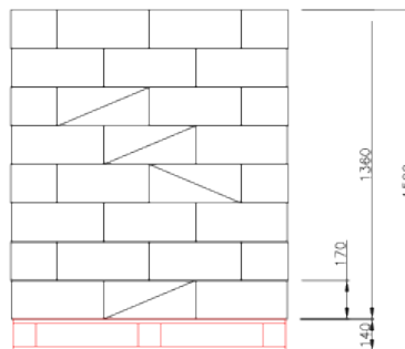
Pallet EPAL
