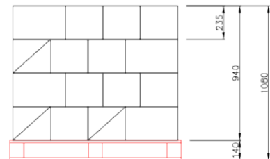
Pallet EPAL
